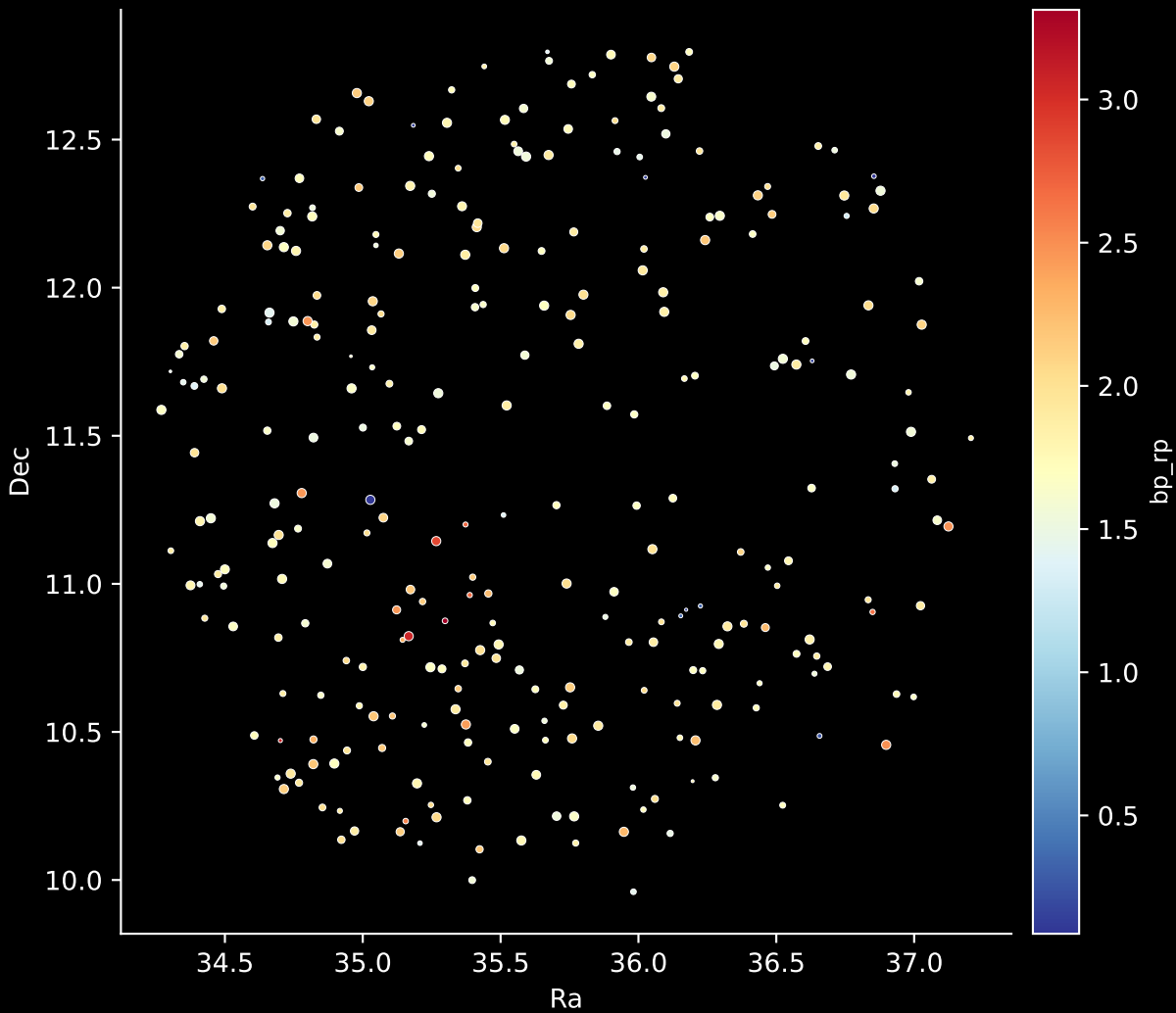
APOGEE DR17 Field: [049-06] Stars: 281
