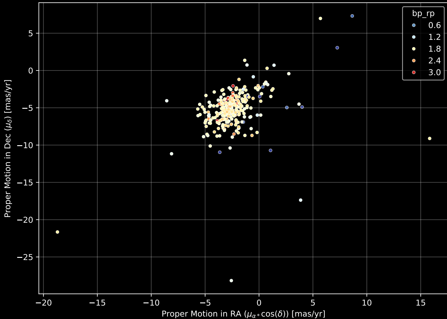
APOGEE DR17 Field: [049-06] Proper Motion Diagram (n= 281)
