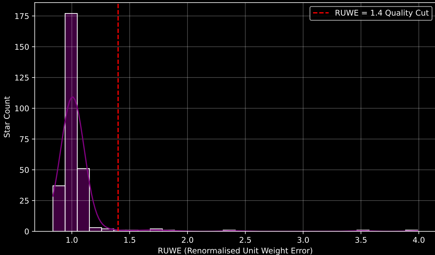
GAPOGEE DR17 Field [049-06] RUWE Distribution (n= 278)
