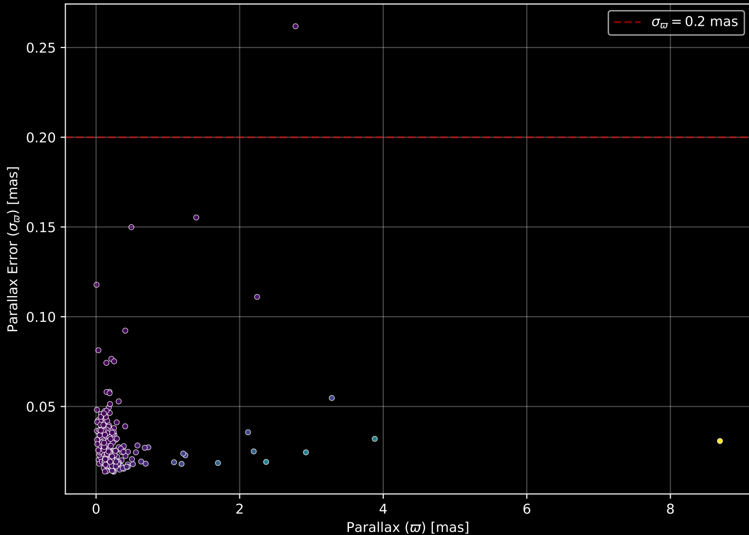
APOGEE DR17 Field: [049-06] Parallax Quality (n= 281)
