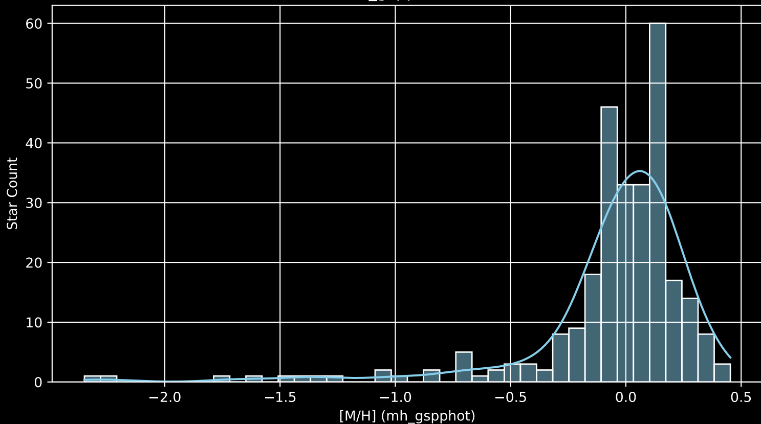
APOGEE DR17 Field: [049-06 [M/H] (mh_gspphot) (n= 278)
